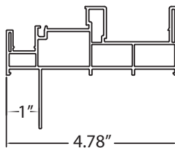
PD1201 FRAME HEAD AND JAMB
